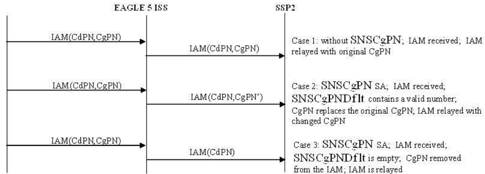
Figure 3-16 ISUP Message Flows for TIF SNS
