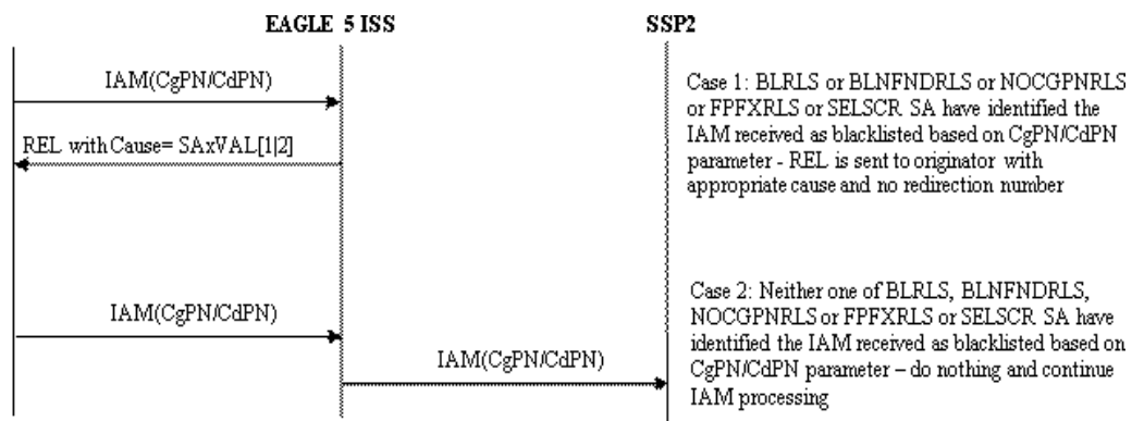
Figure 3-25 TIF Blacklist Basic Message Flow
